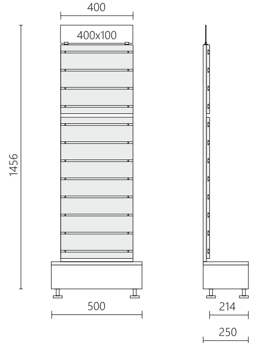
Impulse gondola front
